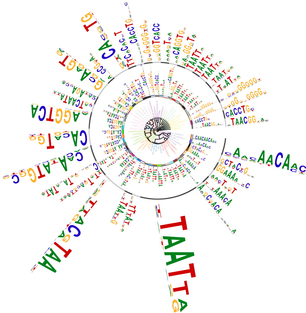
Figure 9: Grouped sequence logo with circos style layout. more color sets with more motifs.
