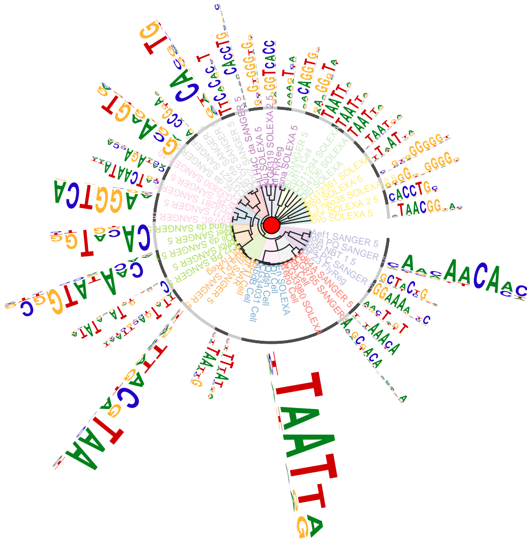
Figure 8: Grouped sequence logo with radialPhylog style layout. Like tag-cloud, the sequence logo size is determined by the number of motifs for the signature. The gray-black circle indicates the range of each signature.
