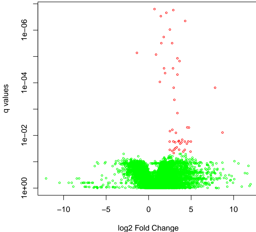
Volcano Plot
