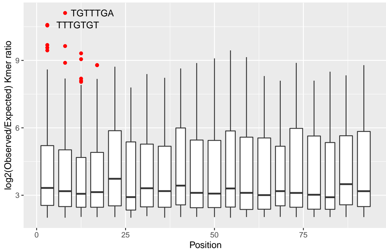
Boxplot of \log_2(\text{Observed/Expected}) Kmer ratio
