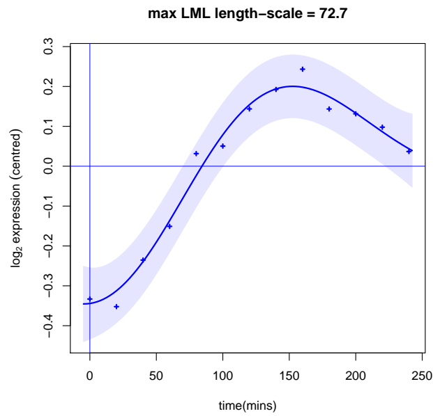
Figure 2: Profile #1 : (a) Log-marginal likelihood (LML) contour. (b) GP fit with maximum LML hyperparameters from the exhaustive search.
